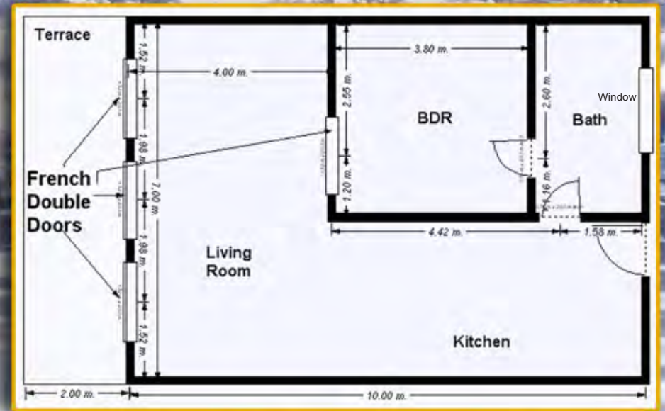
Unit B Plan 70 sm
